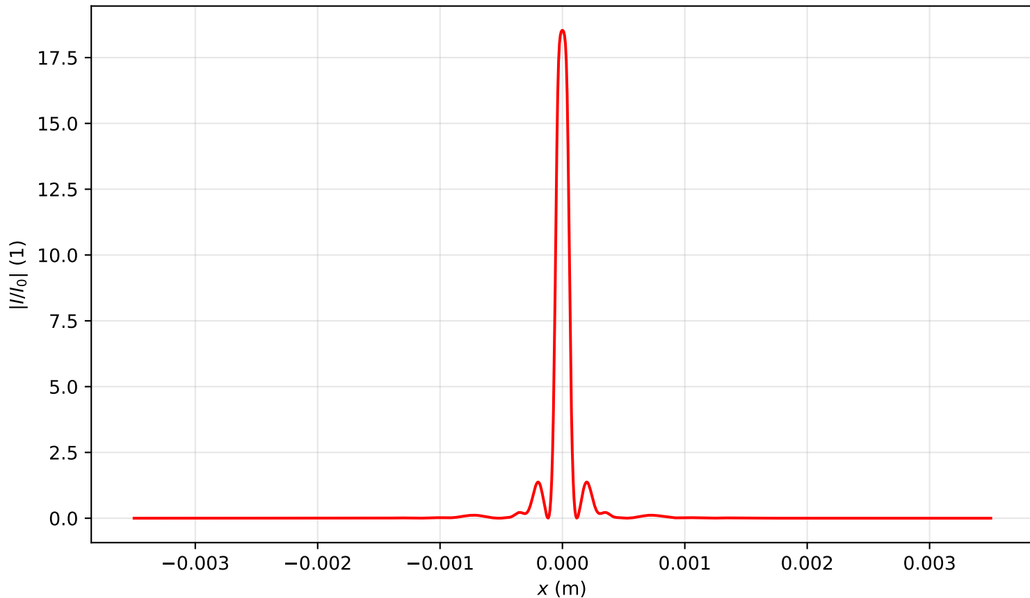
Intensity profile I(x, y = 0, z = 0.955)/I_0 , P_{in}=6.0P_{cr} , artificial time
